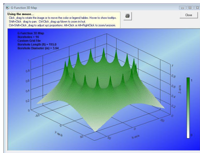
Fig. 4.7 A G Map for a Circular Loopfield
