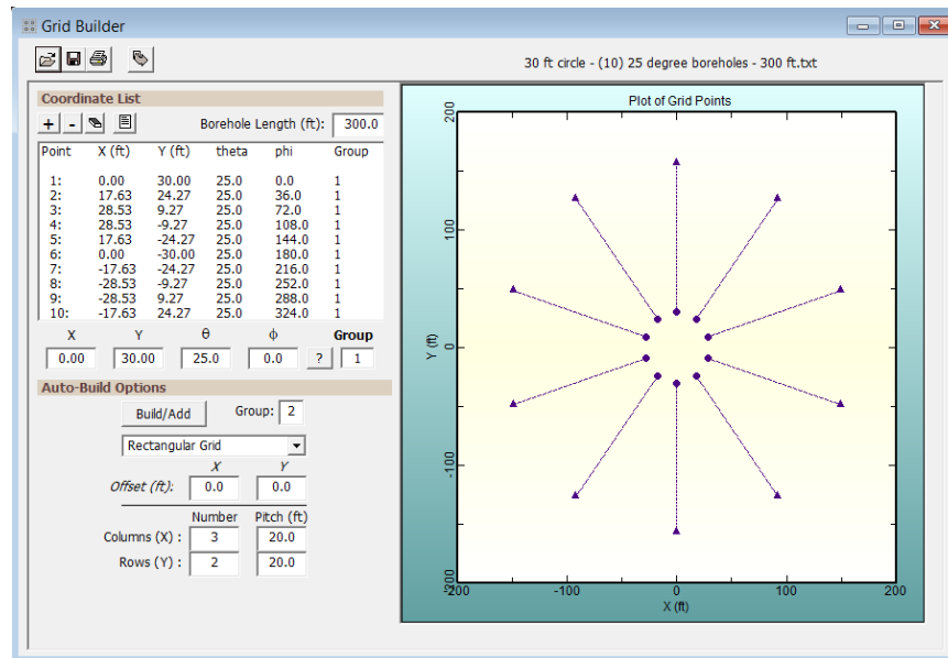
Fig. 4.14B An auto-built angled borehole system
