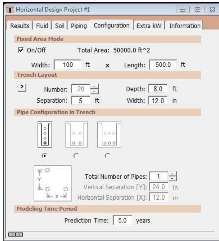
Fig. 5.5 Sample Pit Design
