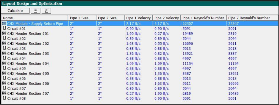
Fig. 11.111 Viewing A Set of Results Well Suited for Purging Design
